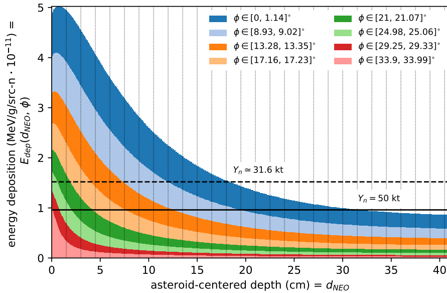
(b) Energy deposition spatial distribution from a \sim 1 MeV neutron source (DPLUS group #21).
