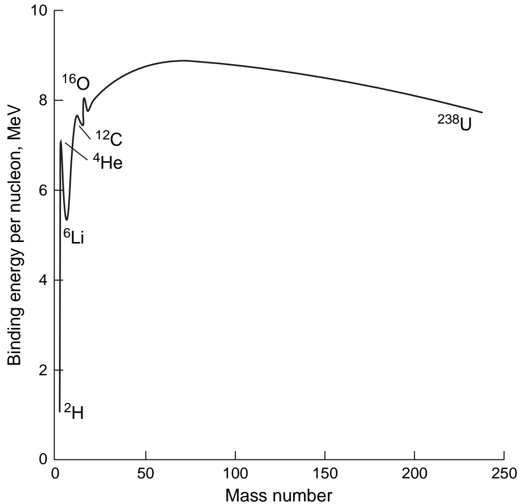
FIGURE 1.1 Curve of binding energy per nucleon. Nuclei with even numbers of protons and neutrons are usually more stable than their odd isotope relatives, which is why the resonance-esque peaks for certain nuclides are shown. Nuclear fission is a process that results in traveling from the far-right towards the center peak of B/A , while nuclear fusion's path is from the far-left up towards the middle. Taken from [76] — this figure was published in “Fundamentals of Nuclear Reactor Physics,” Elmer E. Lewis, pg. 8, Copyright Elsevier (2008). Reprinted by permission of Elsevier.
