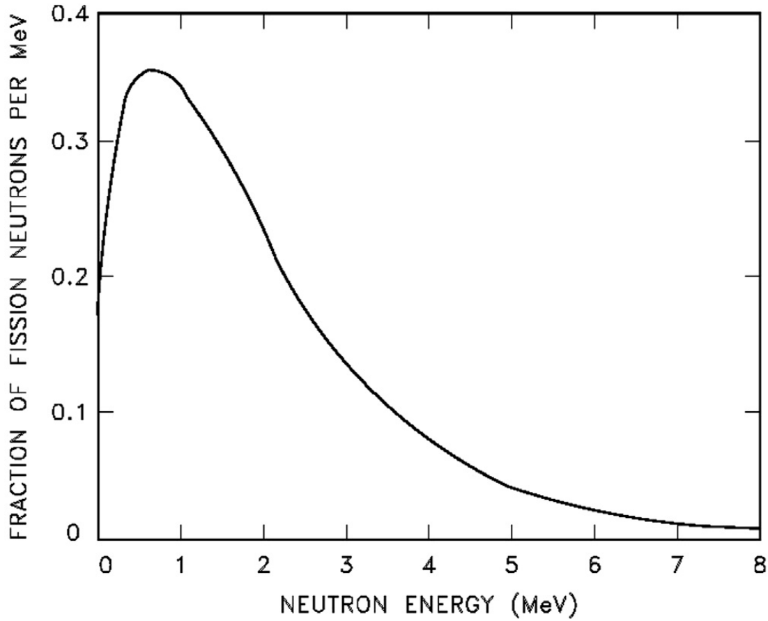
Fig. 4. Neutron energy spectrum produced by the thermal fission of U-235 (DOE HDBK-1019/1-93, 1999). The average energy is 2 MeV while the most probable energy is close to 1 MeV (at the peak). Taken from [80].
